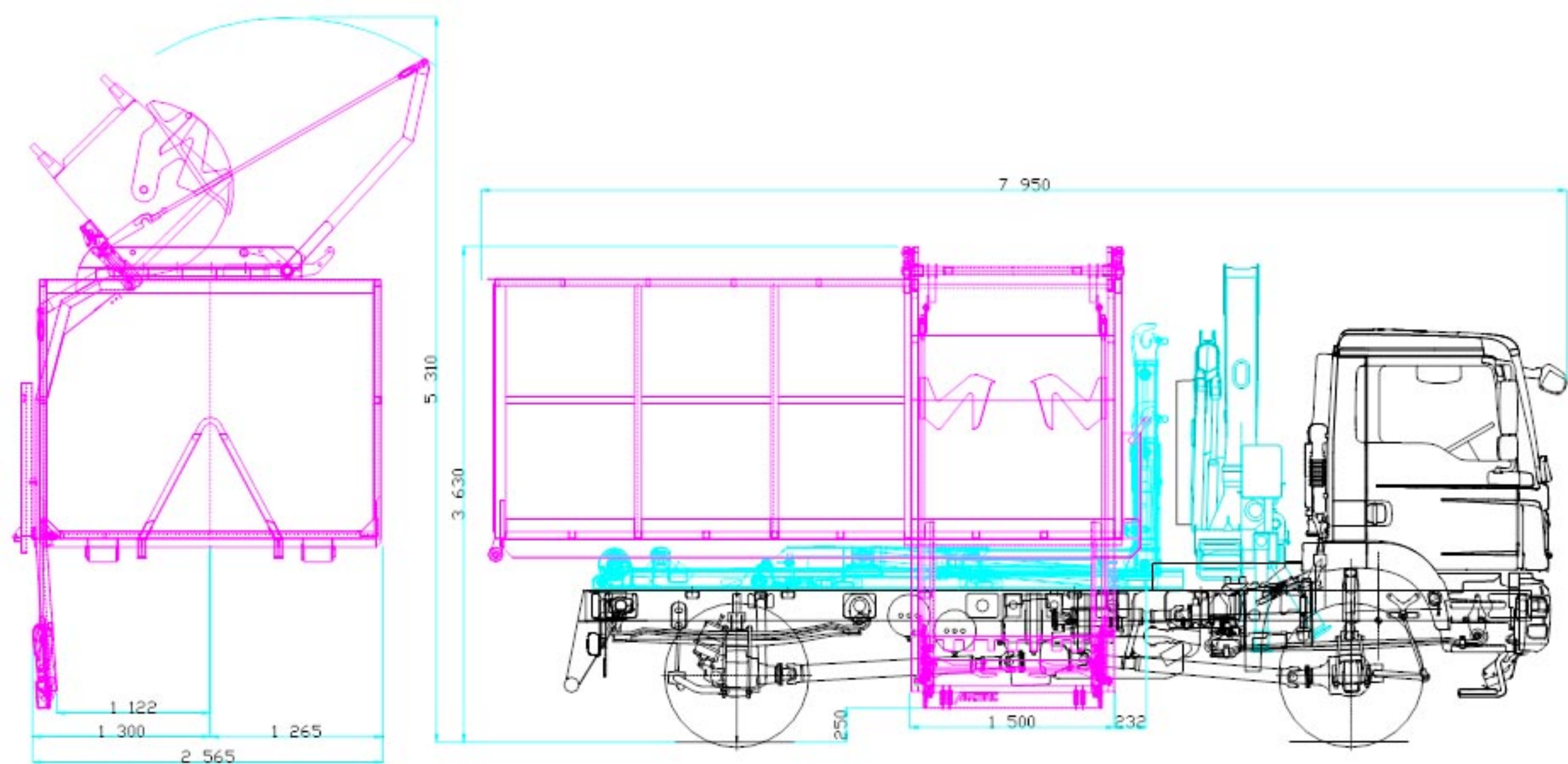
MAN TGM 18.340 4x4 BB 4500mm, Fassi F95A023, Formál NKH12T-400 hák 1000-1570, MULTITEC ABL-460PED1000-20.21V
